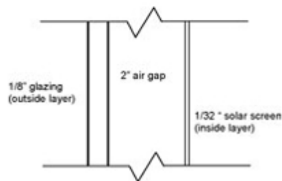
Figure 3 . Window Configuration
